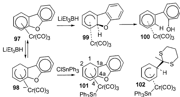
Scheme 26
