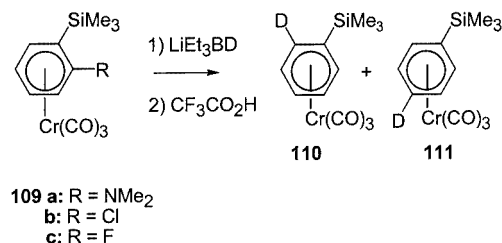
Scheme 29
