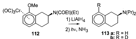
Scheme 30
