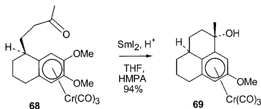
Scheme 19
