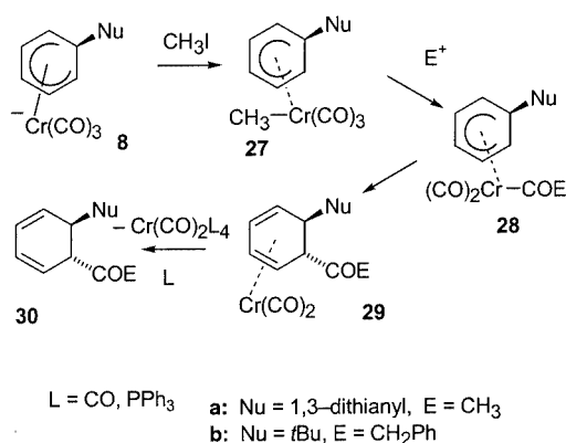
Scheme 10
