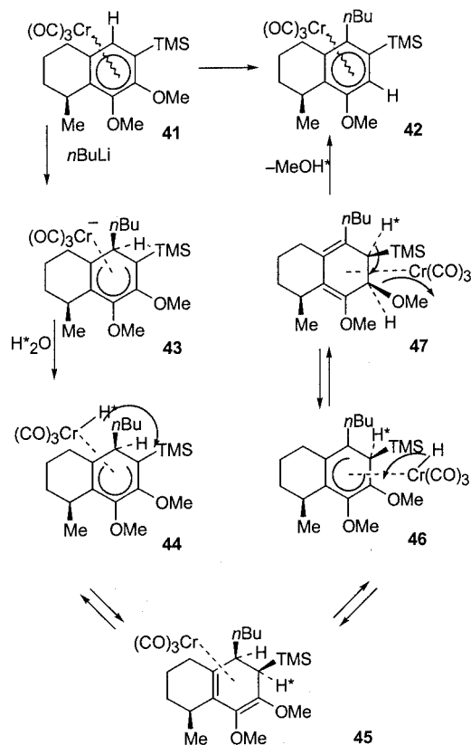
Scheme 14
